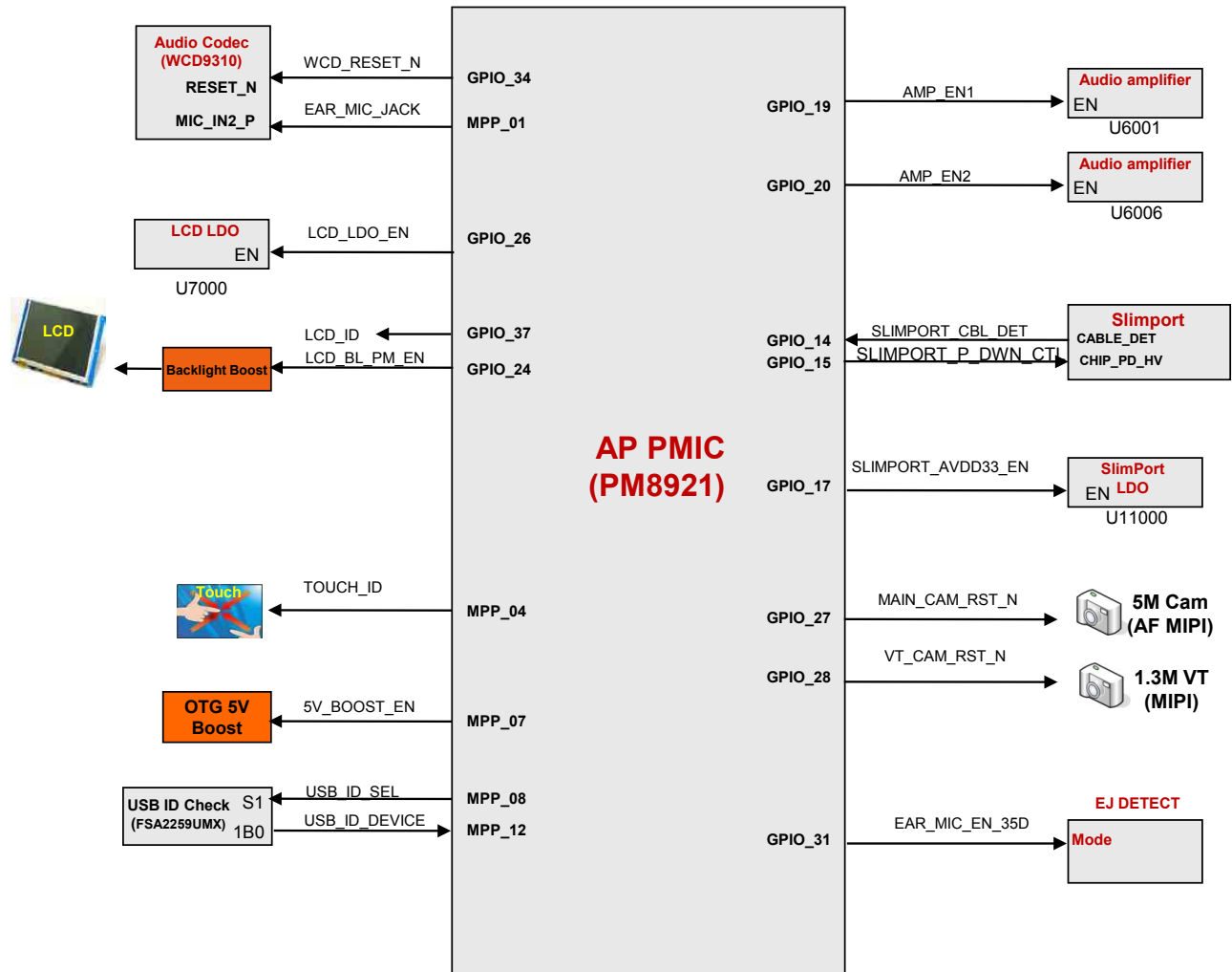
[V500] Block diagram : PM8921 GPIO/MPP INTERFACE
