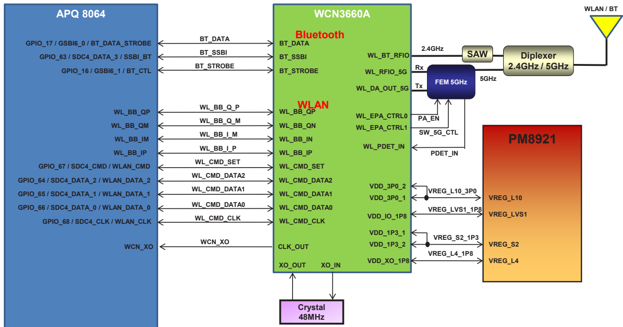
[V500] Block diagram : RF SUB BAND 1 (BT/WI-FI-COB)
