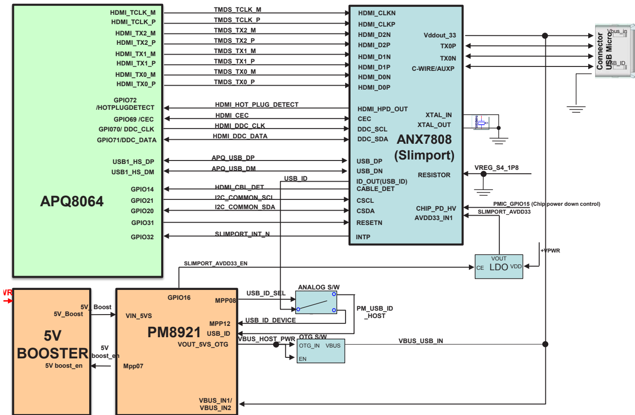
[V500] Block diagram : SLIMPORT/USB OTG
