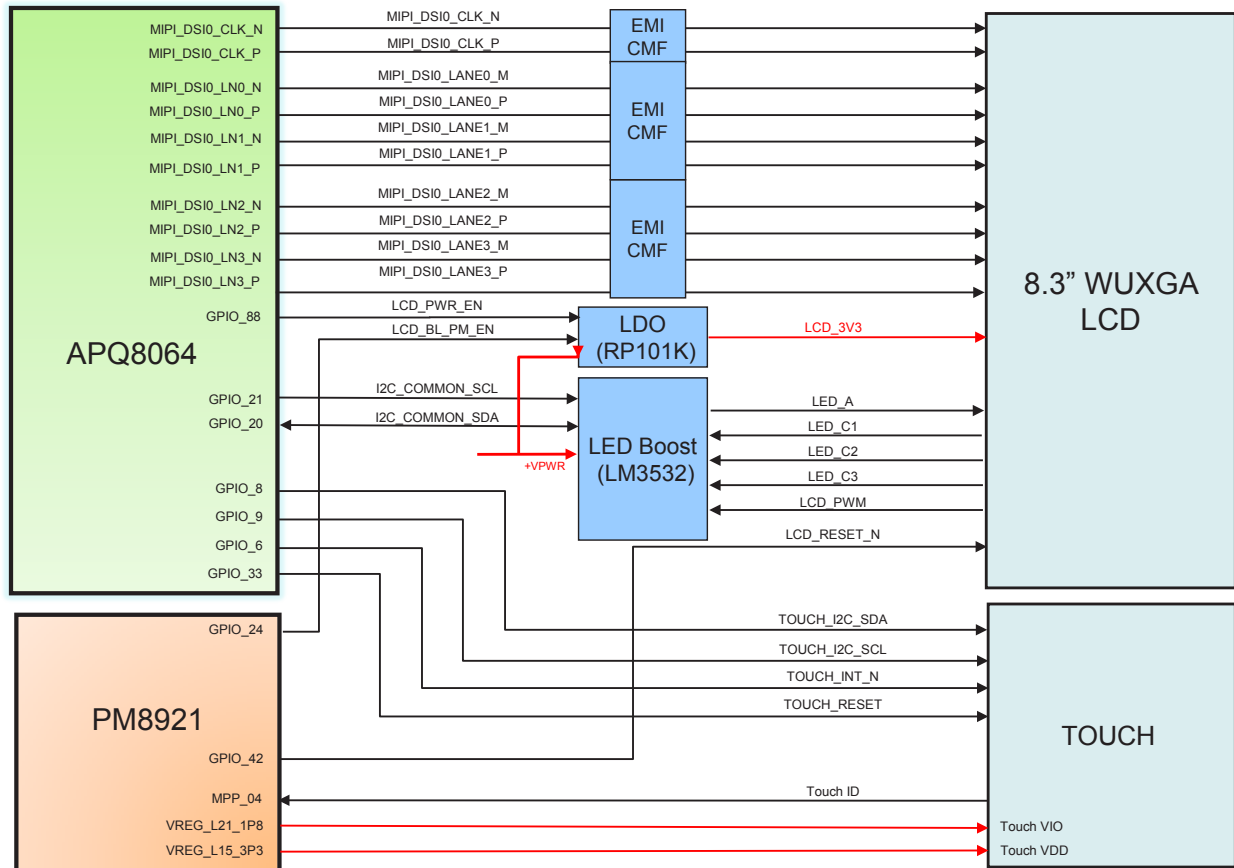
[V500] Block diagram : LCD/TOUCH
