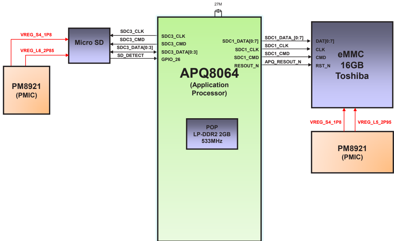
[V500] Block diagram : Memory, Micro-SD
