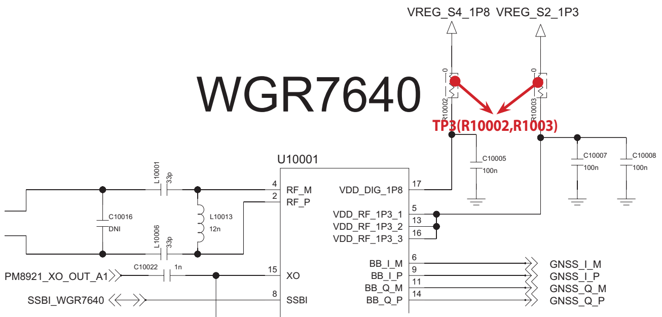
Schematic of GPS Chip(WGR7640)
