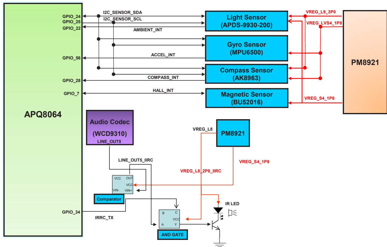
[V500] Block diagram :SENSOR's / IIRC
