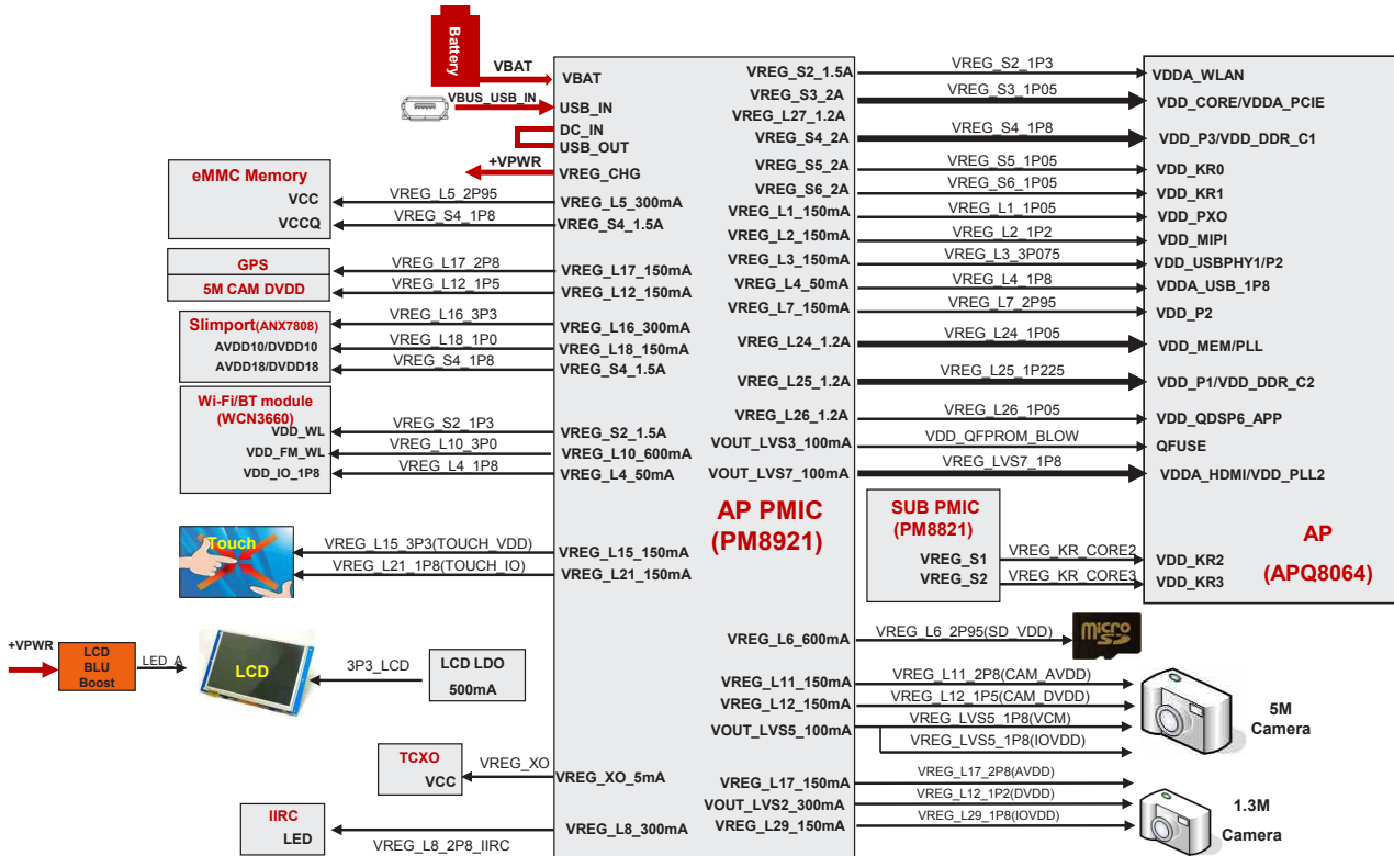
[V500] Block diagram : PM8921 POWER INTERFACE1 _4_4
