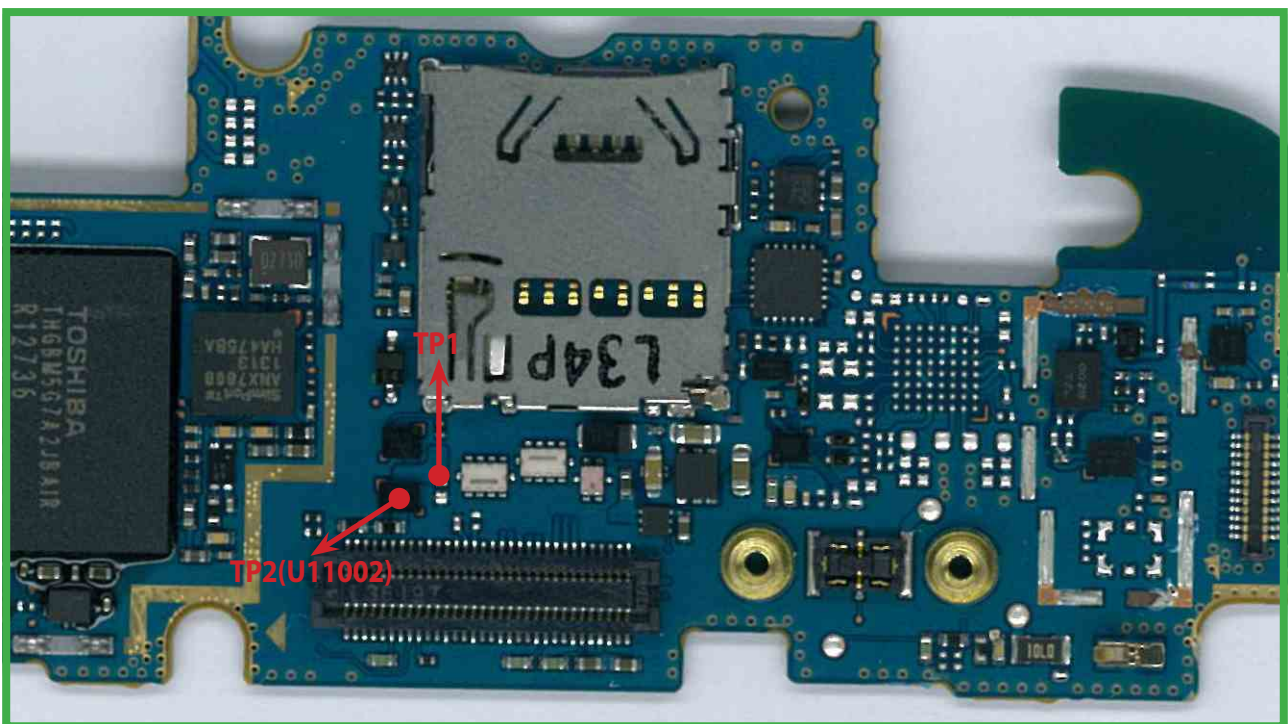
PCB Bottom Side
