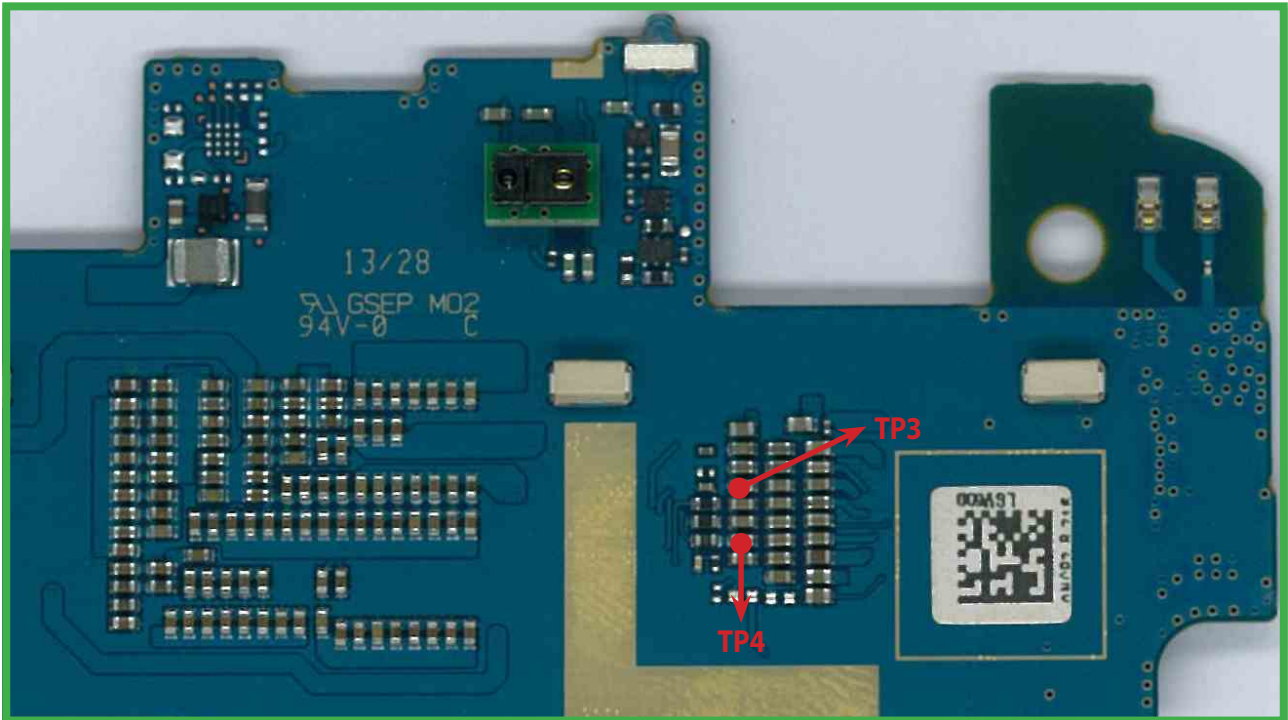
PCB TOP Side
