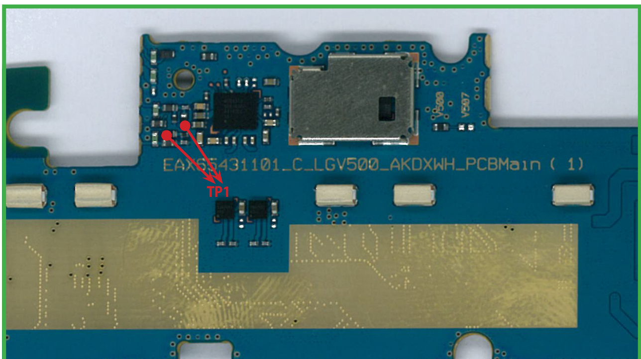
PCB TOP Side
