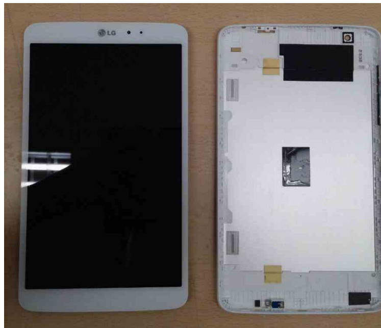
Disassembling direction
