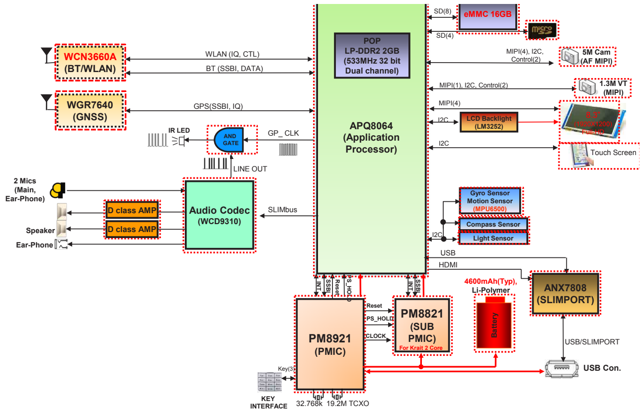
[V500] Total Block Diagram
