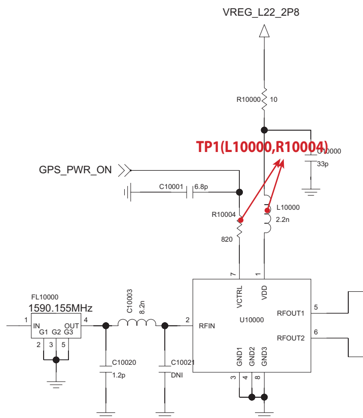
Schematic of External LNA
