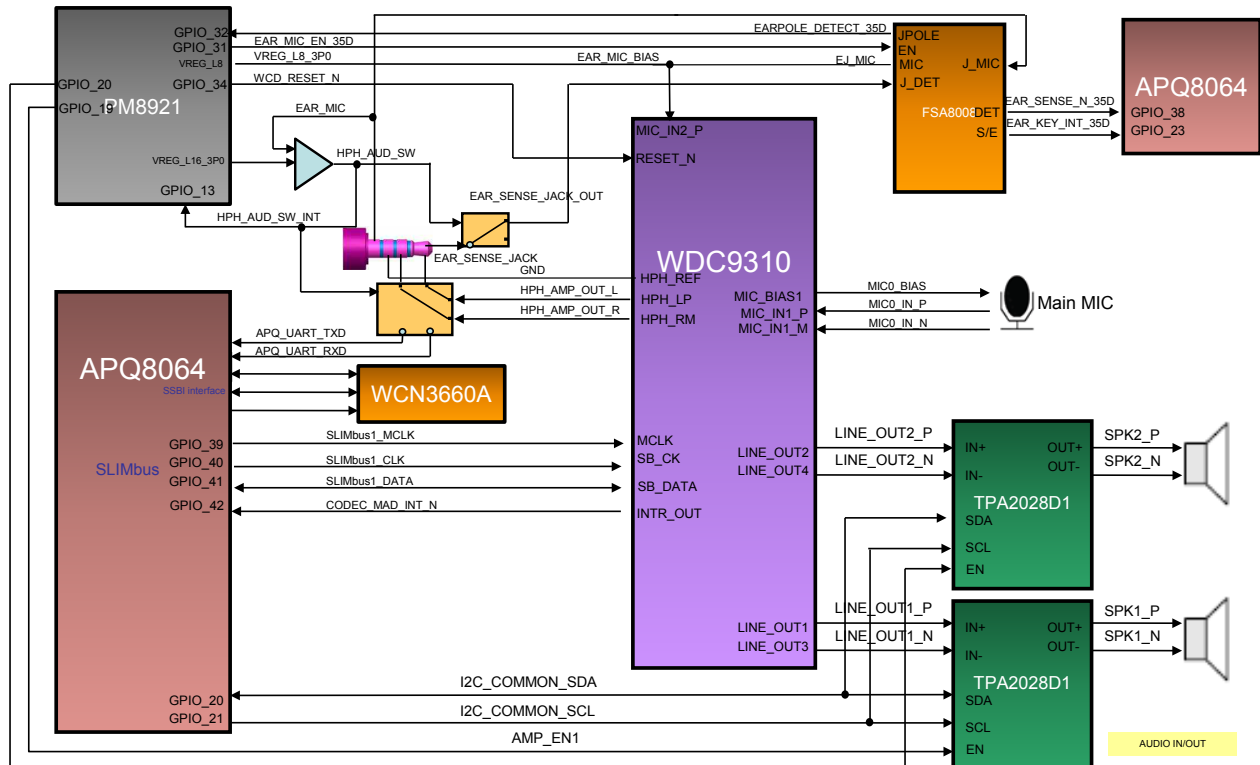
[V500] Block diagram : AUDIO
