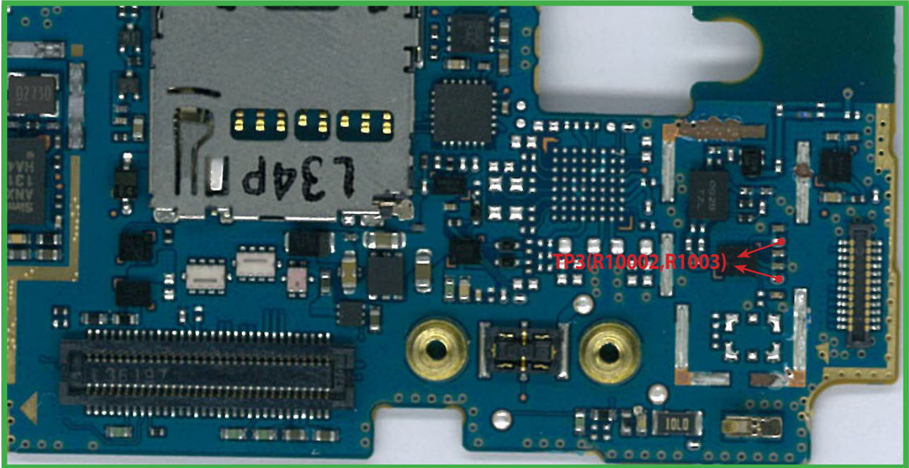
PCB Bottom Side (Inside SMT Type SHIELD CAN)
