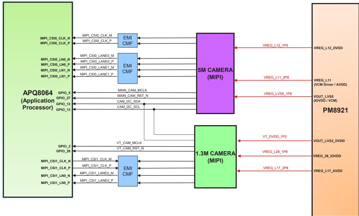
[V500] Block diagram : Camera(5M, 1.3M)
